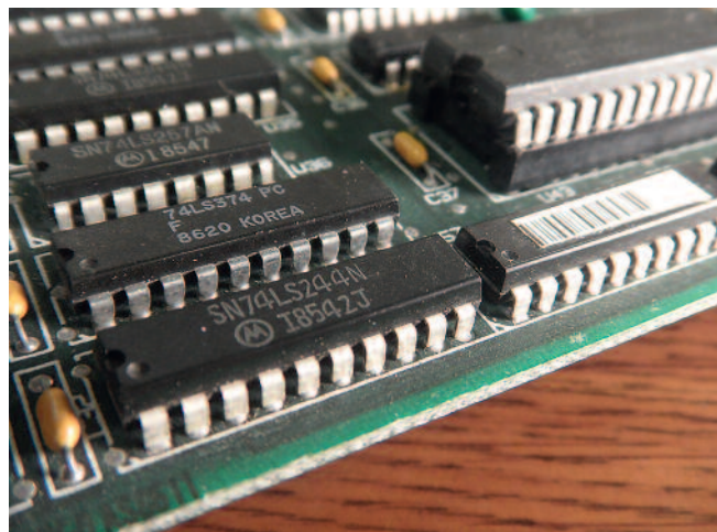
The first through-hole components made their introductions in the commercial applications in the late 1960s – the integrated circuits were embedded in the black plastic housings of the "chips" and the circuits were connected with the long metal legs of the chips, which commonly have 16 to 20 legs (photos: MicroCare Corp.)
