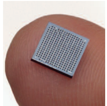
BGA components evolved away from space-wasting legs, and all electrical connections are under the chip, using micron-sized dots of solder to complete the circuits – BGA designs also increase exponentially the number of connections that can be made, since the number of possible connections is limited by the area of the chip, not the perimeter
